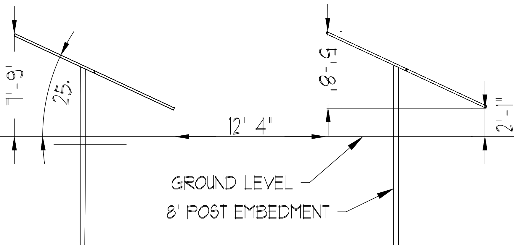
Typical Array
